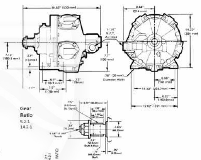
MM Series Motor Dimensions
